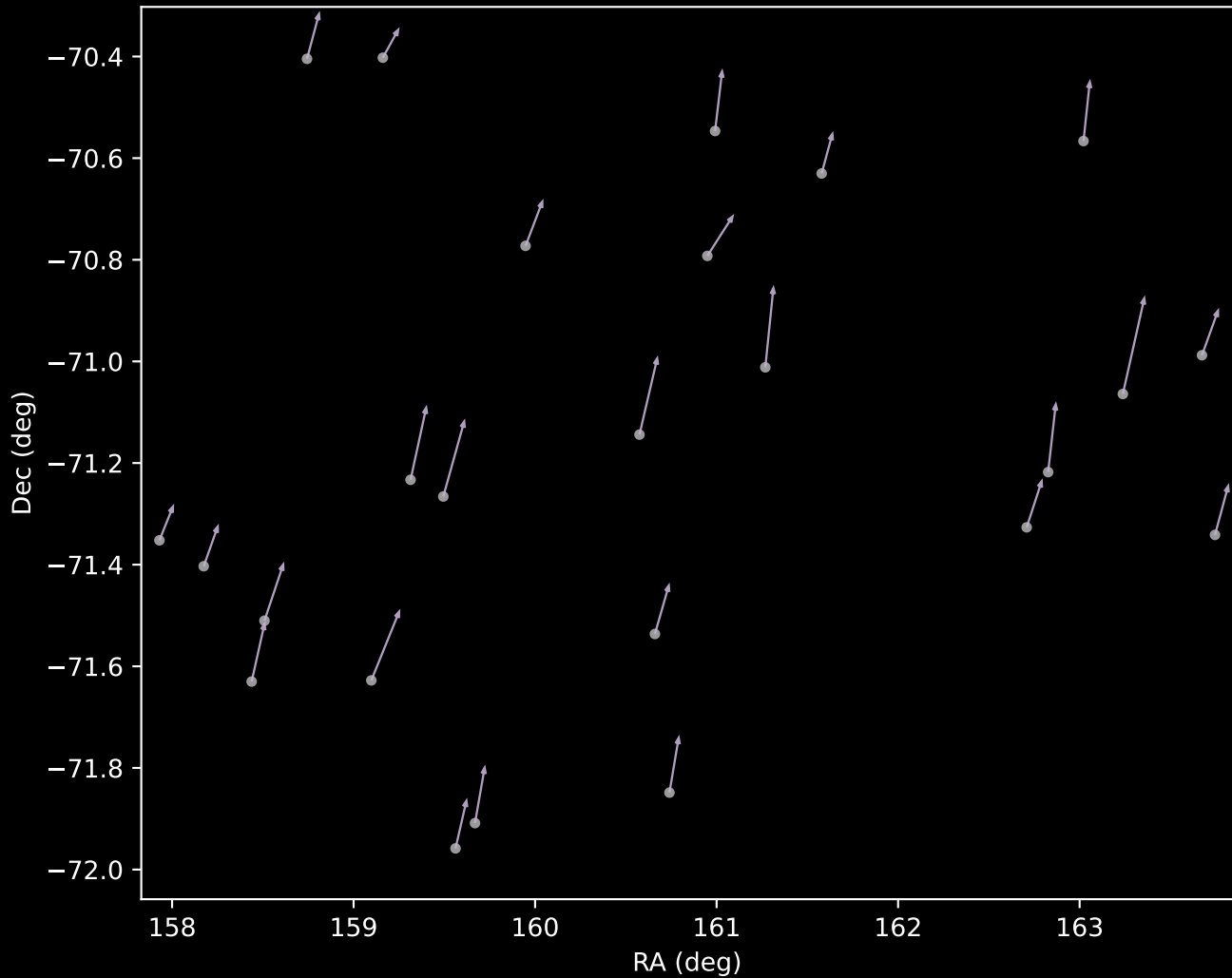
GALAH DR4 Cluster 9 Proper Motion Vectors (n=25)
