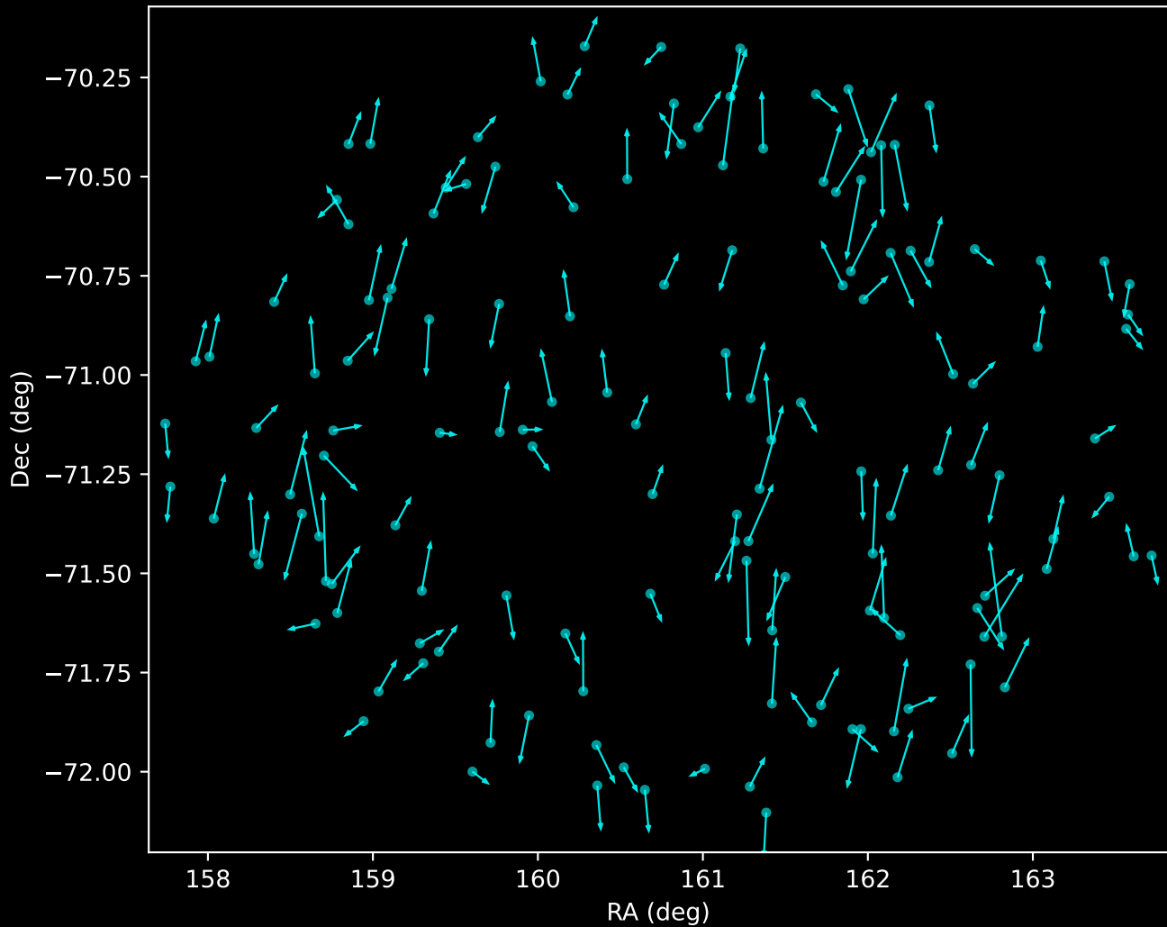
GALAH DR4 Noise Stream Proper Motion Vectors (n=144)
