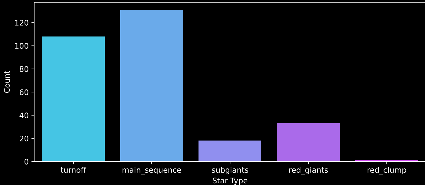
GALAH DR4 Field: [287] Count plot of Star Type
