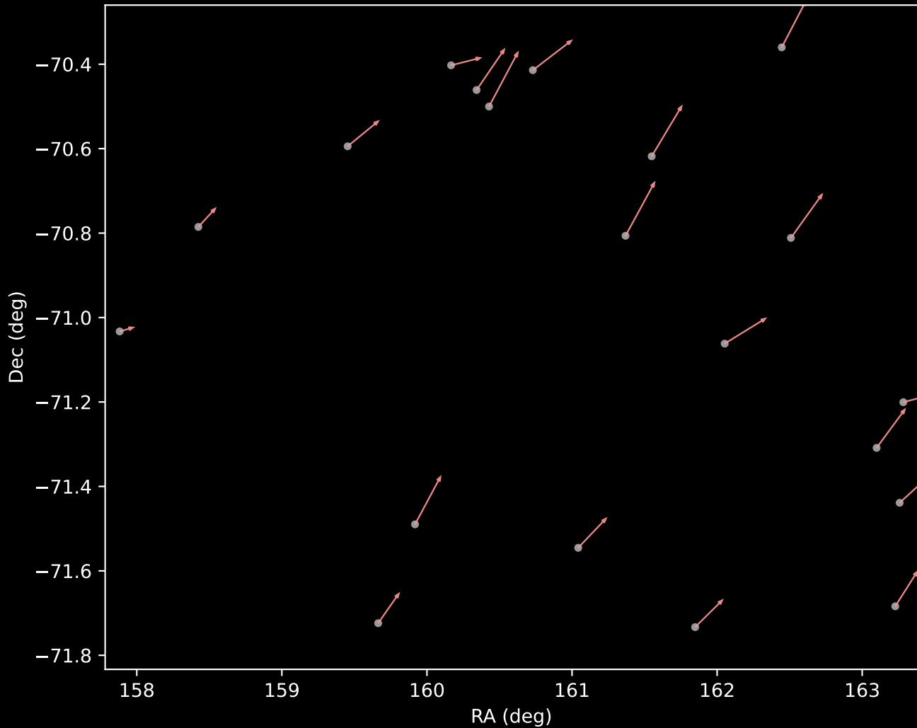
GALAH DR4 Cluster 7 Proper Motion Vectors (n=20)
