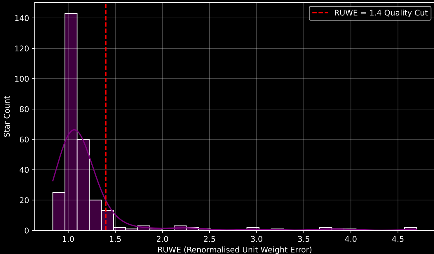
GALAH DR4 Field [287] RUWE Distribution (n= 283)
